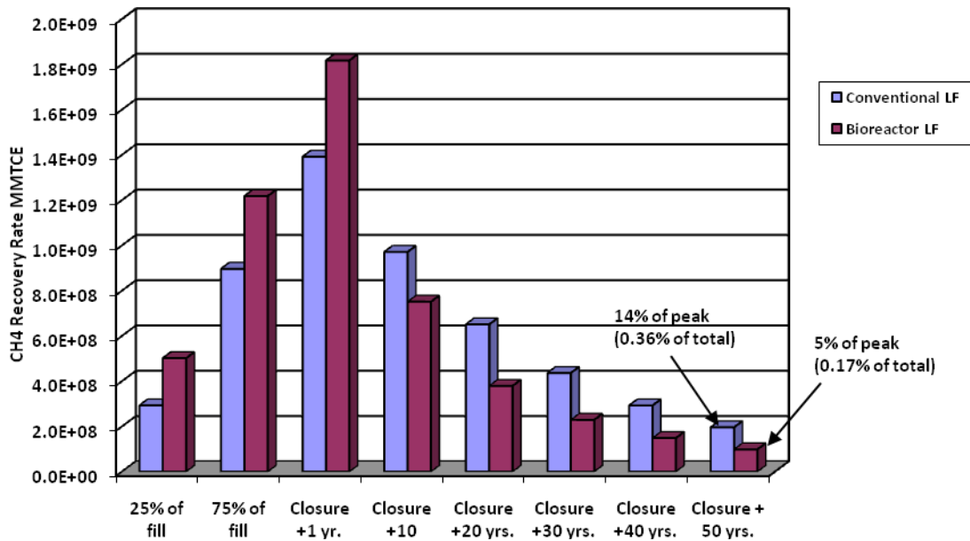
Figure 5-1. Methane Recovery Rates, Conventional vs. Bioreactor
